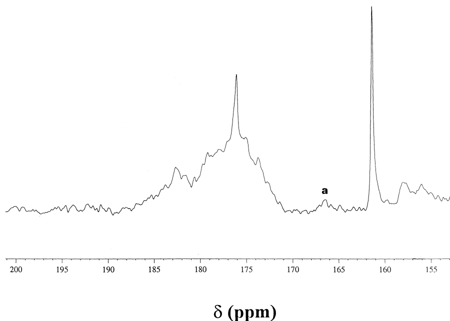
Fig. 5. 150 MHz ^{13}\text{C} NMR spectrum of \text{Ti}_2\text{Tf} (1.5 mM, 10% \text{D}_2\text{O} , HEPES buffer 50 mM, \text{pH}^* 7.4 ) in the presence of 6 mM ^{13}\text{C} -enriched \text{NaH}^{13}\text{CO}_3 . The signal labeled a is assigned to \text{Ti}_2\text{Tf} -bound synergistic anion.
